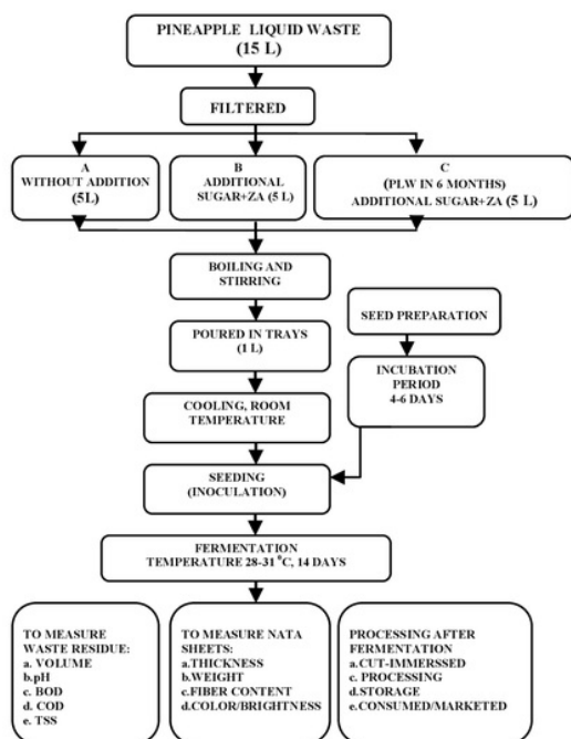
Figure 1. General Scheme of Nata Making (Adapted [19])
